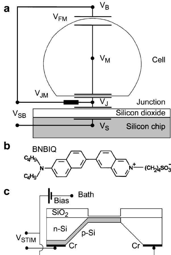
FIG. 1. Silicon-to-cell stimulation. (a) A cell (diameter about 20 \mu\text{m} ) is attached to oxidized silicon, separated by a film of electrolyte (thickness about 50 nm). The silicon dioxide, the attached membrane, and the free cell membrane are described by capacitors, the film of electrolyte by an Ohmic resistor. A voltage V_{SB} is applied between chip and bath. The voltage transients V_{JM} and V_{FM} across the attached and free membrane are converted to fluorescence transients by a voltage-sensitive dye. (b) The amphiphilic hemicyanine dye BNBIQ is adsorbed to the outer surface of the cell membrane. (c) Chip. The p -doped stimulation area is insulated with 50 nm \text{SiO}_2 . It is contacted from the back through an etched and p -doped pyramidal well at chromium pads. Voltage pulses V_{STIM} between stimulation spot and bath are applied through a bias voltage.
